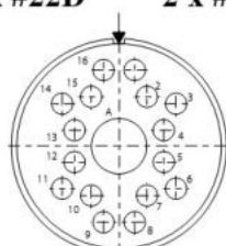
19A-17 1 x #8 20 x #16
