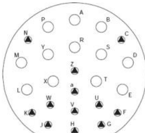
25-24 12X #12/12X #16
