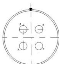
19-4 4 x #8
