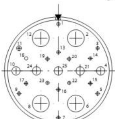
25-26 4 x #8 16 x #20 5 x #12
