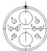
17-60 2 x #8 8 x #22D
