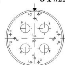
19-18 4 x #8 14 x #22D
