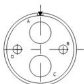
17-22 2 x #8 2 x #12
