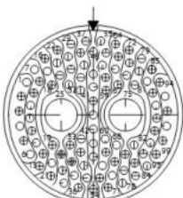
25-7 2 x #8 97 x #22D
