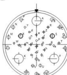
25-41 3 x #8 22 x #22D 3 x #20 11 x #16 2 x #12
