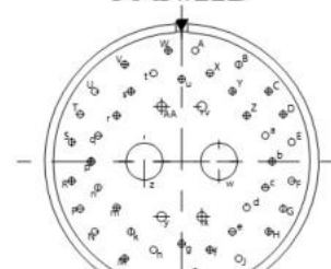
25-17 6 x #8 36 x #22D
