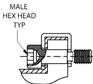
MALE HEX HEAD TYP NON-FLOATING JACKSCREW SYM. HJ OPTION
