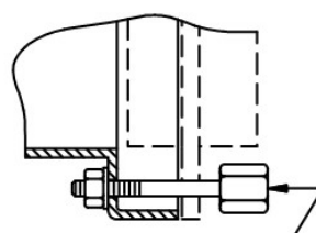
FEMALE JACKPOST D THREAD - TYP SYMBOL F
