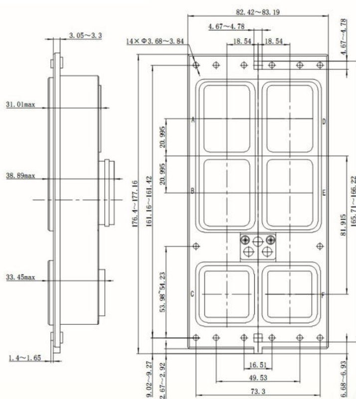
Equipment Receptacle
